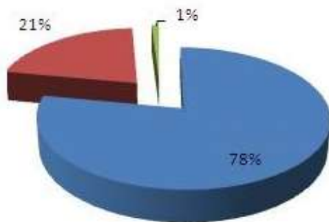
Composition of Air
